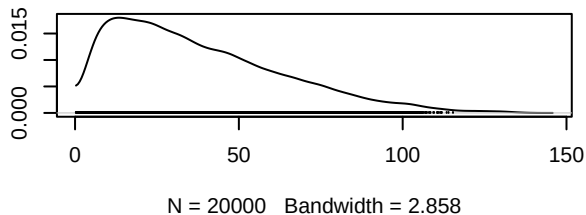
Density of d.Gefitinib.Almonertinib
