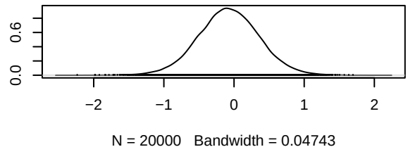
Density of d.chemo.Afatinib
