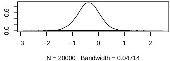
Density of d.Afatinib.Placebo
