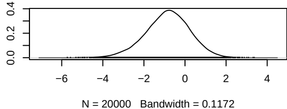
Density of d.Osimertinib.Osimertinib_antiangi
