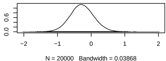
Density of d.chemo.Erlotinib
