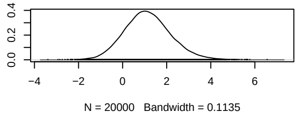
Density of d.Afatinib.Afatinib_Cetuximab
